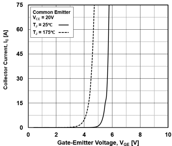
Figure 3. Transfer Characteristics
